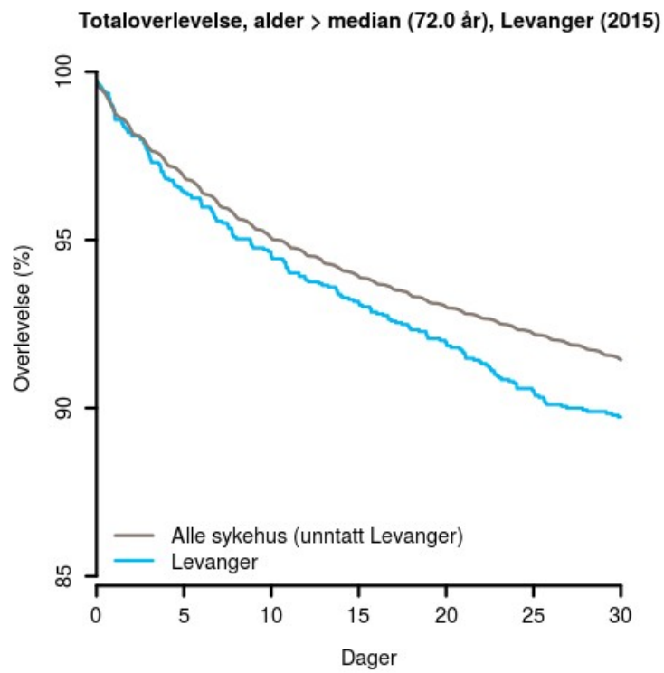
Figur 2 : Kaplan-Meierkurver for totaloverlevelse, alder > median (72.0 år), Levanger (2015)
