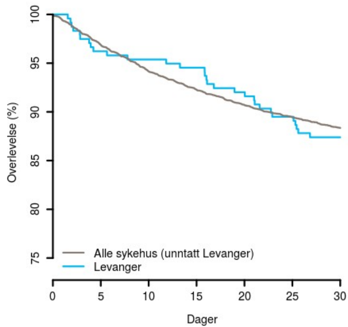
Figur 6 : Kaplan-Meierkurver for hoftebrudd, alder > median (84.0 år), Levanger (2013-2015)
