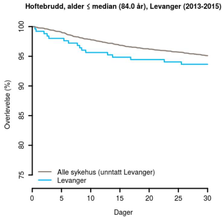
Figur 5 : Kaplan-Meierkurver for hoftebrudd, alder \leq median (84.0 år), Levanger (2013-2015)
