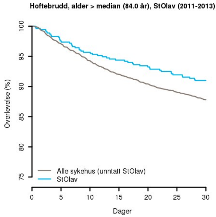
Figur 6 : Kaplan-Meierkurver for hoftebrudd, alder > median (84.0 år), StOlav (2011-2013)
