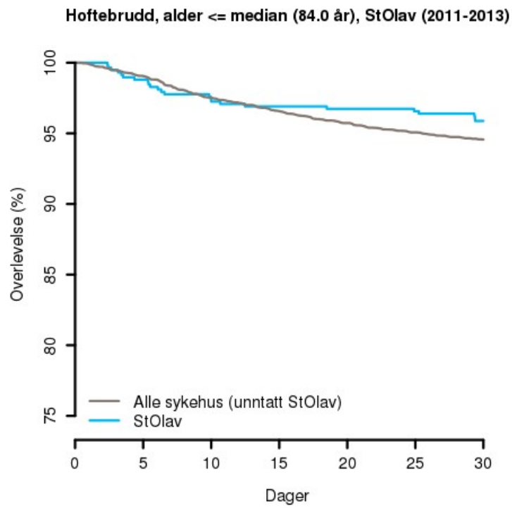
Figur 5 : Kaplan-Meierkurver for hoftebrudd, alder \leq median (84.0 år), StOlav (2011-2013)
