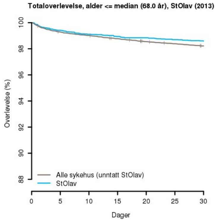
Figur 1 : Kaplan-Meierkurver for totaloverlevelse, alder <= median (68.0 år), StOlav (2013)
