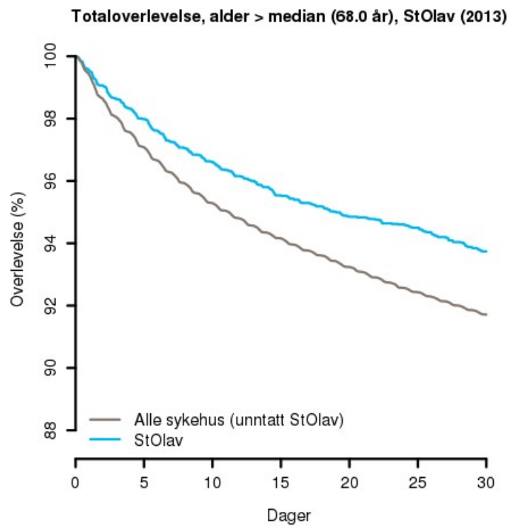
Figur 2 : Kaplan-Meierkurver for totaloverlevelse, alder > median (68.0 år), StOlav (2013)
