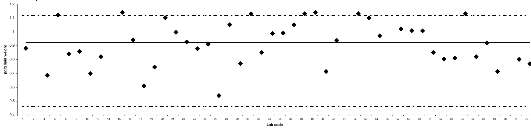
2,3,4,6,7,8-HxCDF
