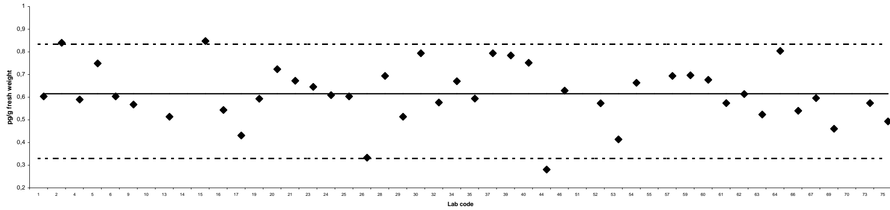
2,3,4,6,7,8-HxCDF
