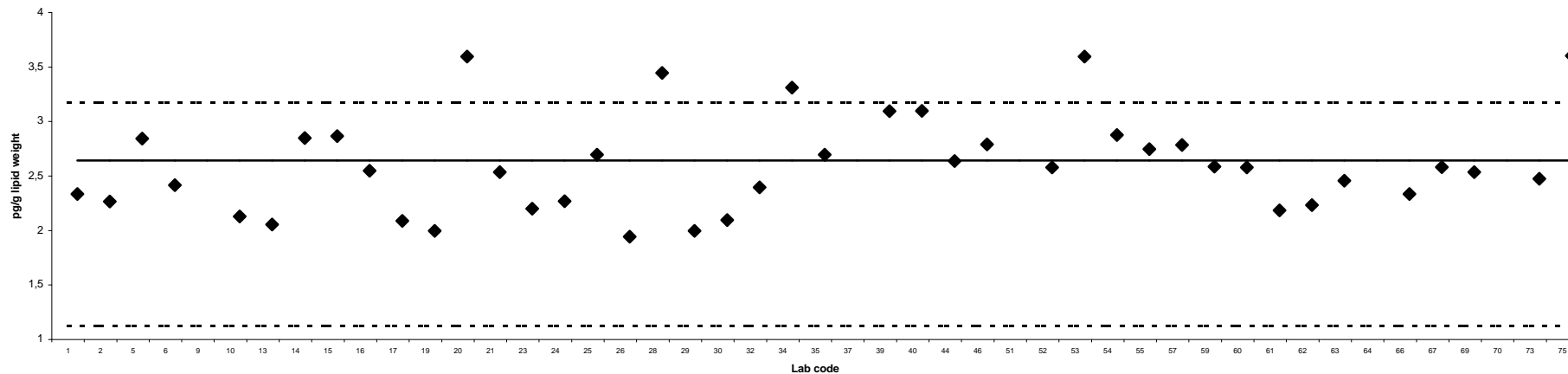
2,3,4,7,8-PeCDF
