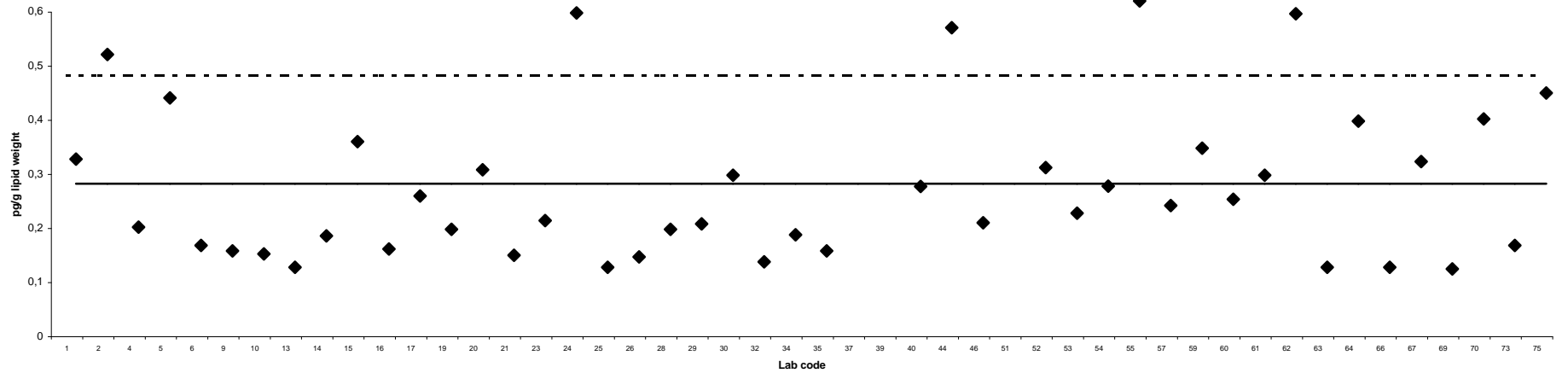
1,2,3,4,7,8,9-HpCDF
