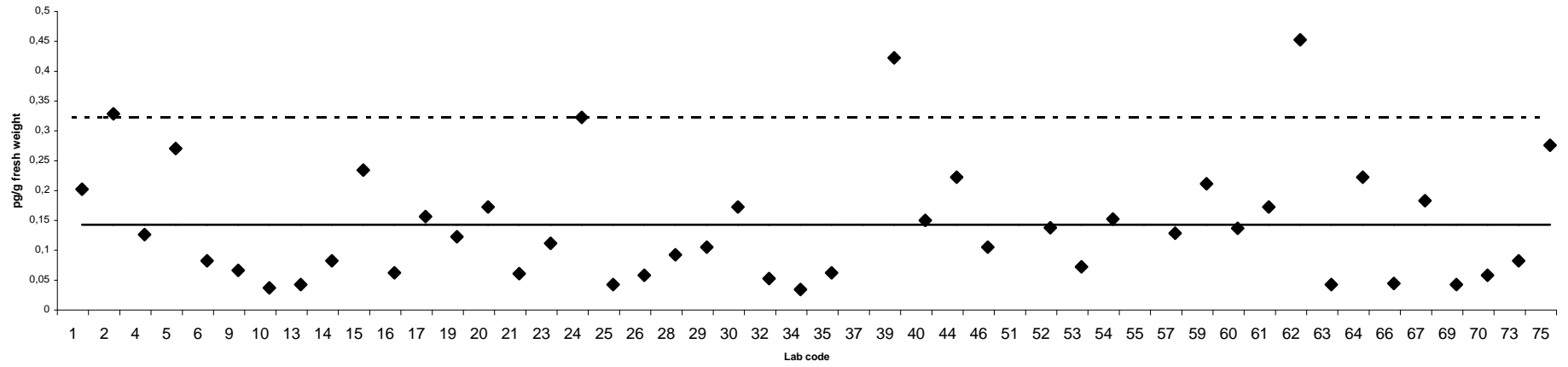
1,2,3,4,7,8,9-HpCDF
