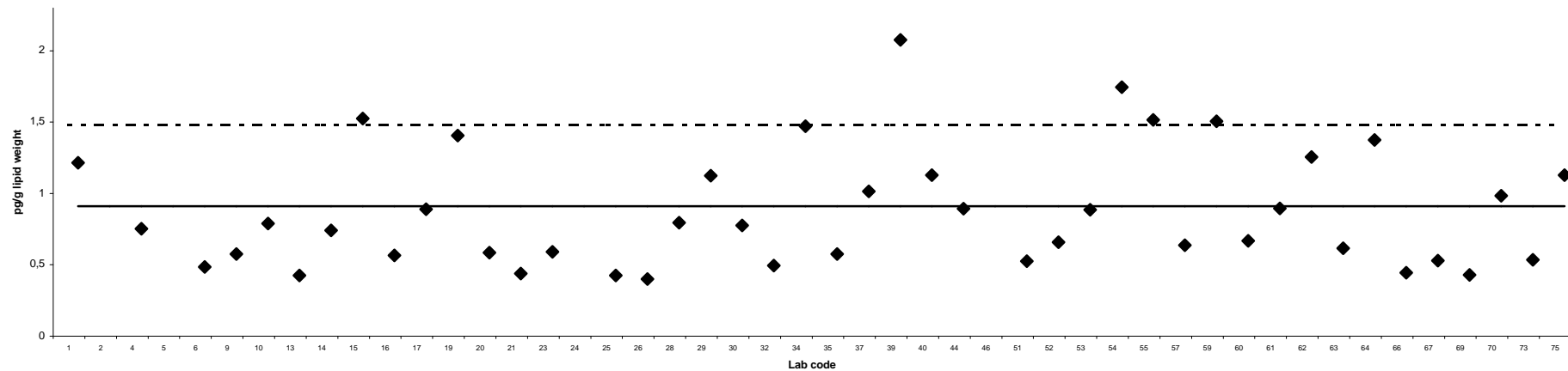
1,2,3,4,6,7,8,9-OCDF
