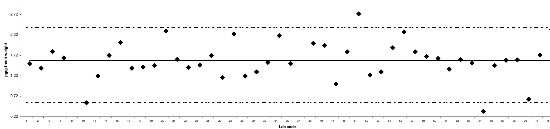
2,3,4,7,8-PeCDF
