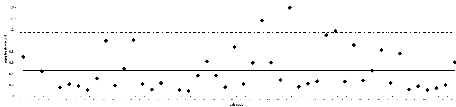
1,2,3,4,6,7,8,9-OCDF
