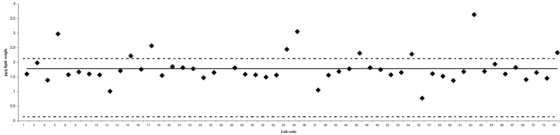
1,2,3,6,7,8-HxCDF
