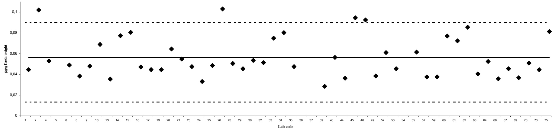
1,2,3,4,6,7,8-HpCDF
