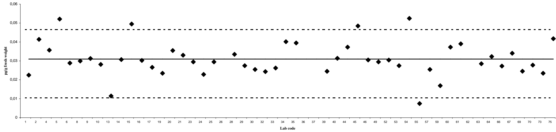
1,2,3,6,7,8-HxCDF
