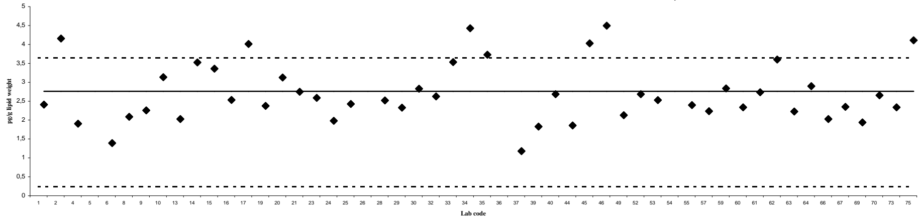
1,2,3,4,6,7,8-HpCDF
