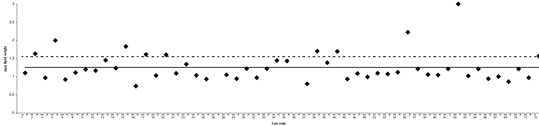
2,3,4,6,7,8-HxCDF
