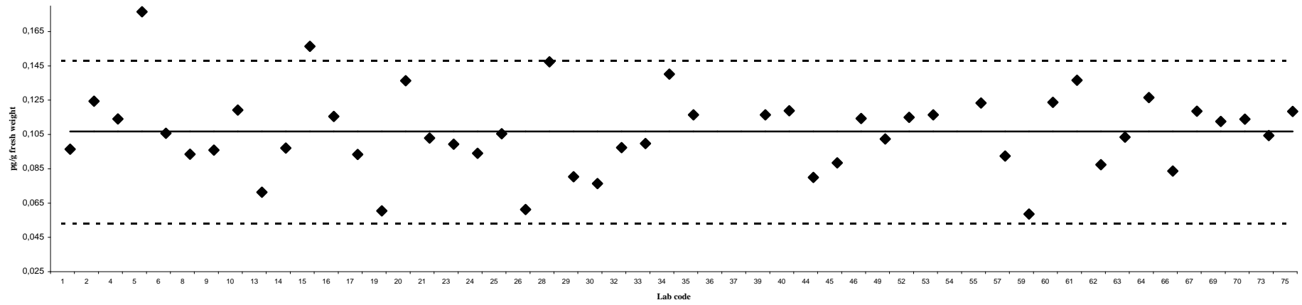
2,3,4,7,8-PeCDF
