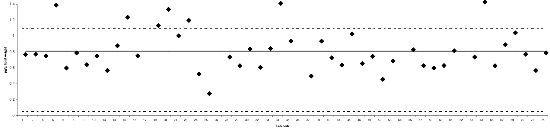
2,3,7,8-TCDF
