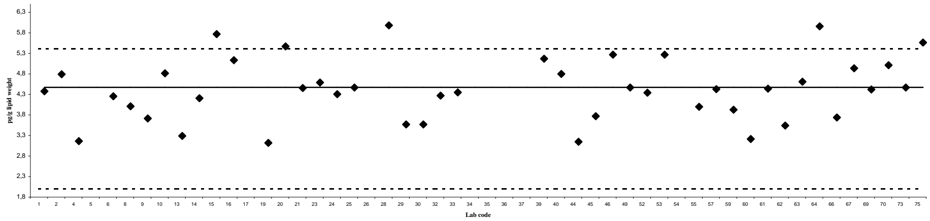
2,3,4,7,8-PeCDF
