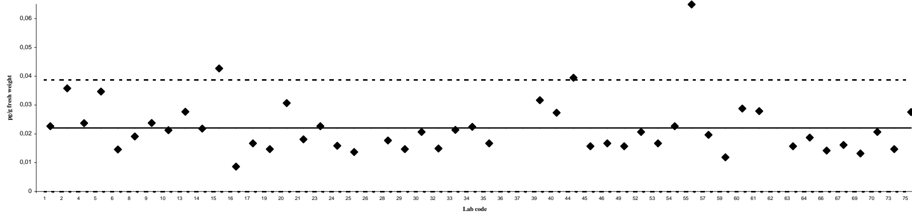
2,3,4,6,7,8-HxCDF
