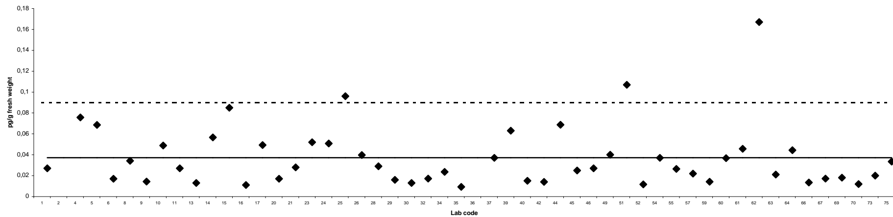
2,3,7,8-TCDF
